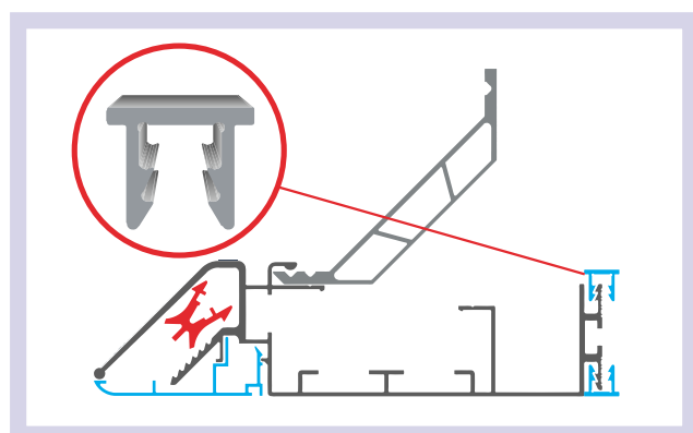
AL klips2 ID VINYL DVSHT125.170T0,08P1146 Clip for double-sided box - 0.25 Euro/pcs
