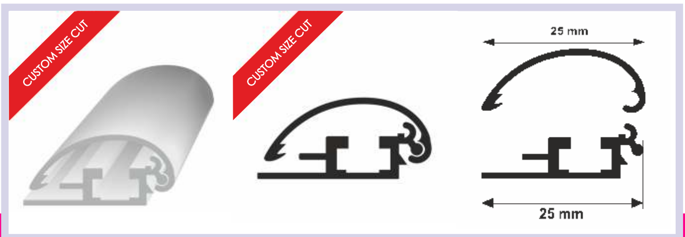
25 mm aluminum snap profile Price: 3.90 Euro/m
