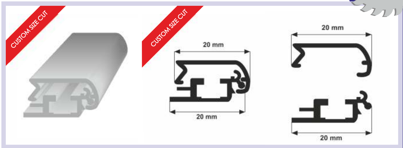
20 mm aluminum snap profile Price: 3.40 Euro/m
