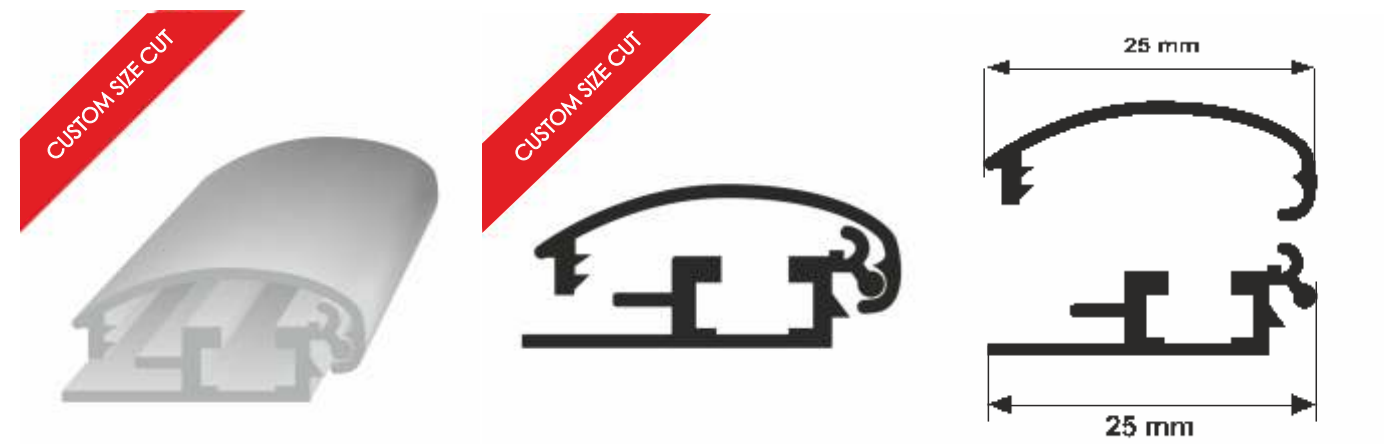
25 mm aluminum snap profile Price: 3.90 Euro/m
