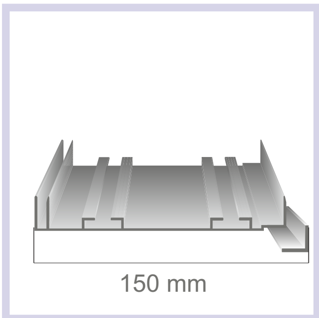
ID PL150T0,954P1909 Raw look - 9,80 Euro/m
